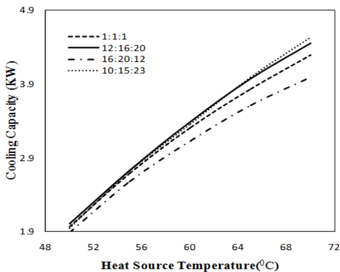
Fig. 3. Effect of heat source temperature on cooling capacity
