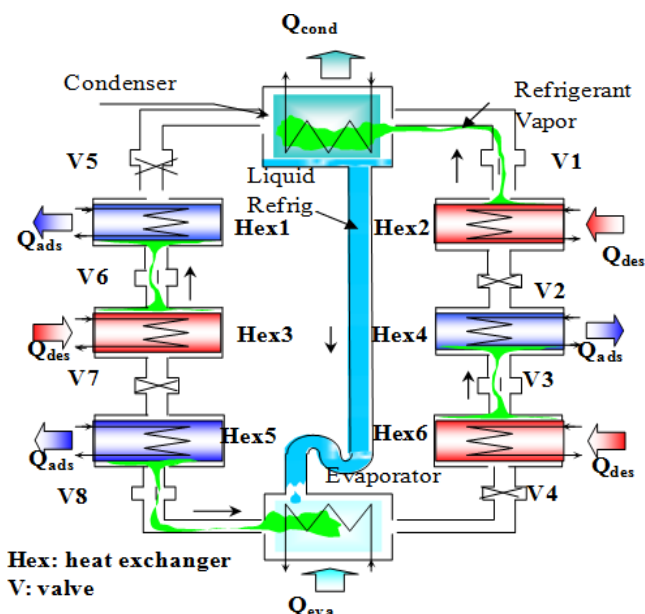
Fig. 1 Schematic diagram of the three-stage adsorption chiller.
