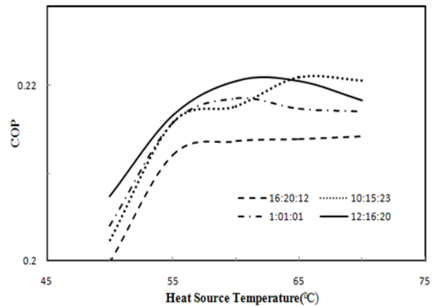
Fig. 4 Effect of heat source temperature on COP
